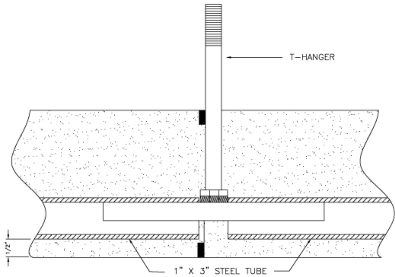
ROOF SUPPORT DETAIL
